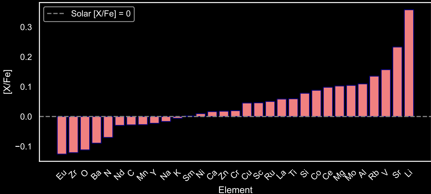
Abundance Pattern for GALAH Main Sequence Stars: Star Field [90] (N=72)
