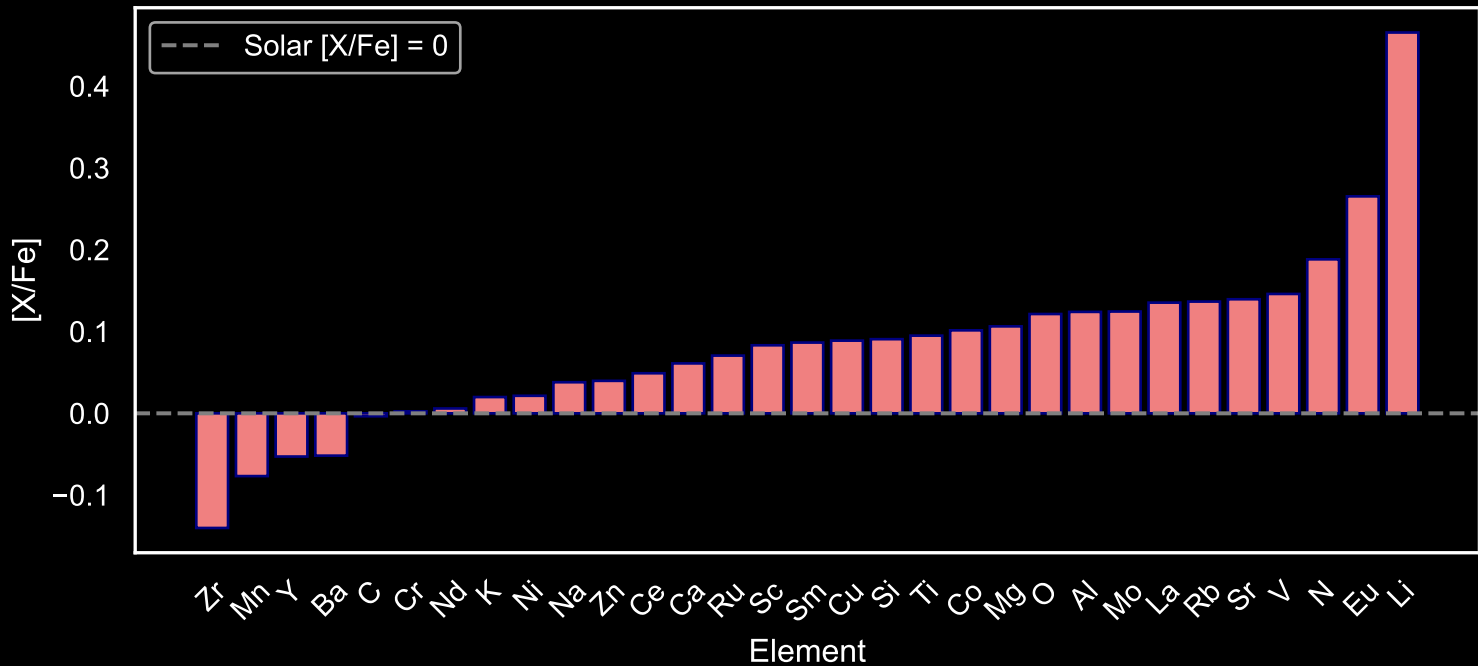
Abundance Pattern for GALAH Star Field [90] (N=210)
