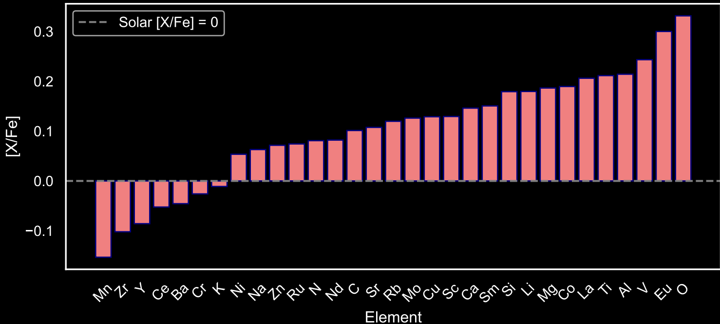
Abundance Pattern for GALAH Red Giants: Star Field [90] (N=60)
