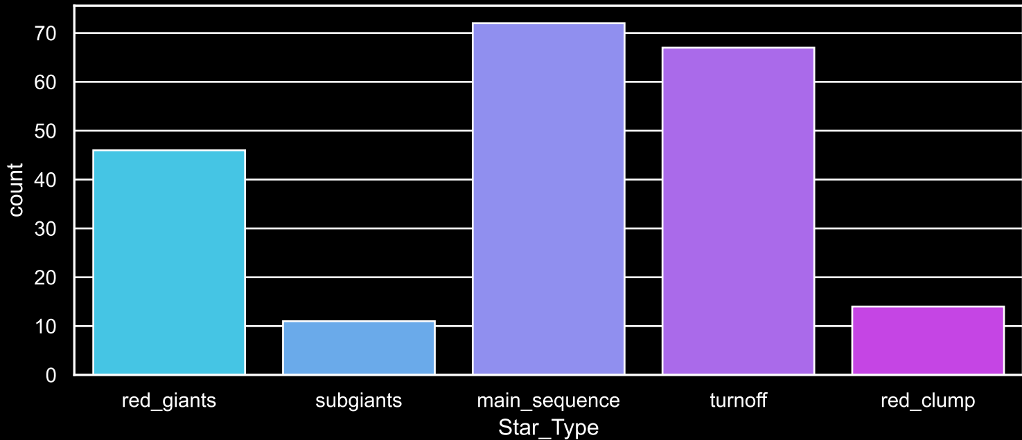
Field [90] Count plot of Star Type
